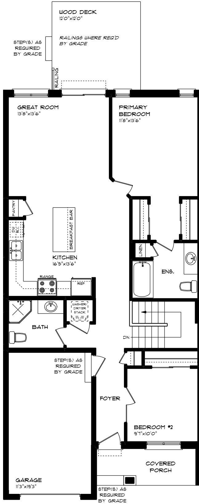
ARBOR (ESSENTIAL SPECS) LOT 42B (#8) FINCH STREET MAIN FLOOR PLAN 9' MAIN FLOOR CEILING APPROX. 1,132 SQ. FT.
